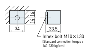
[Terminal part]
