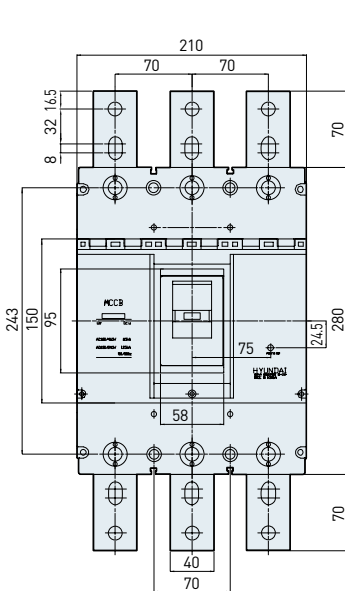
[Terminal part]
