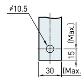
[Connection conductor]
