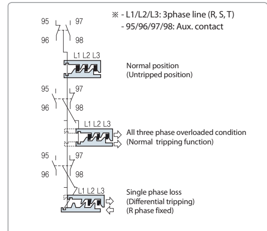
Tripping function
