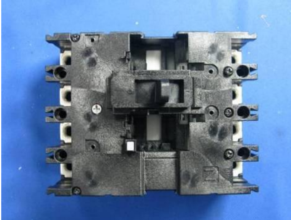
Open view, 4P, MCCB
