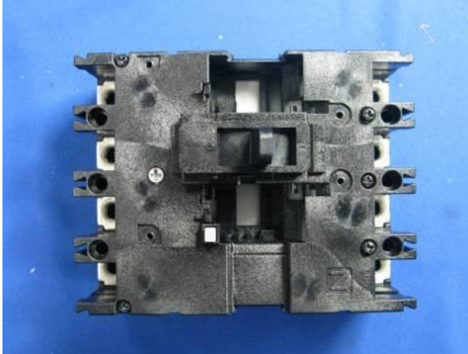
Open view, 3P + N, MCCB
