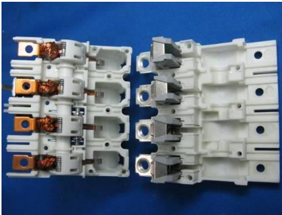
Box of contact, 3P + N, MCCB
