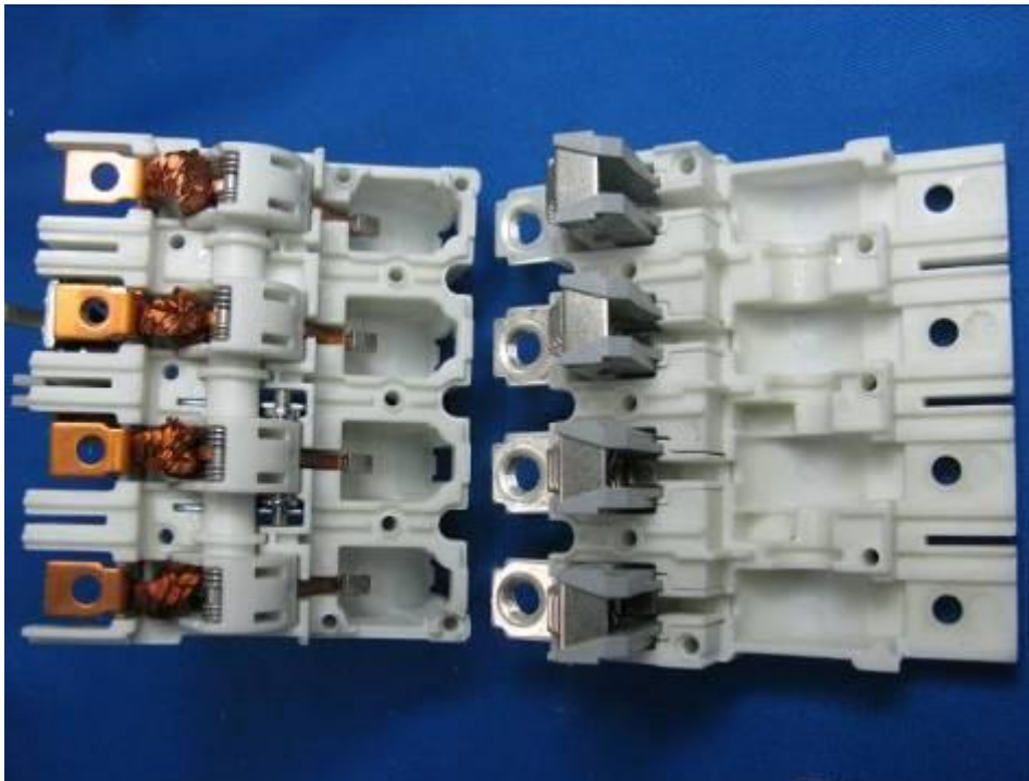
Box of contact, 4P, MCCB
