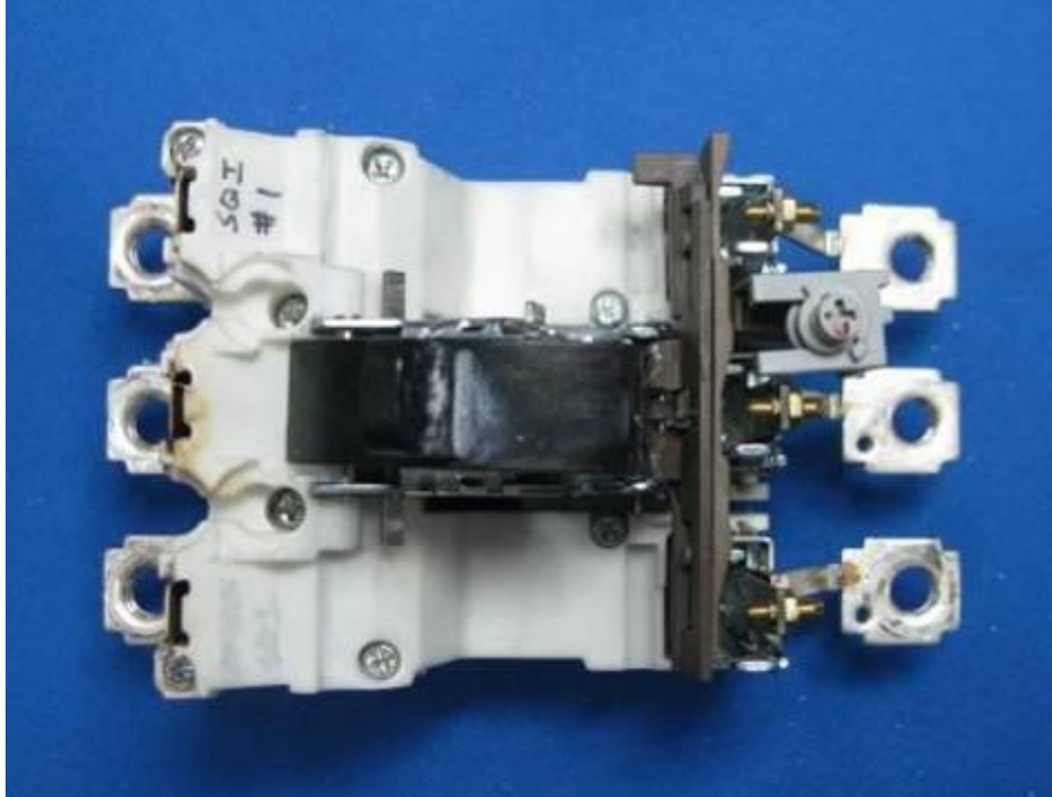
Open view, 3P, MCCB
