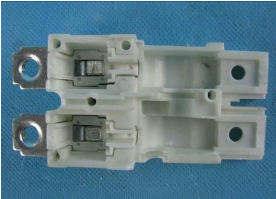
Box of contact, 2P, MCCB
