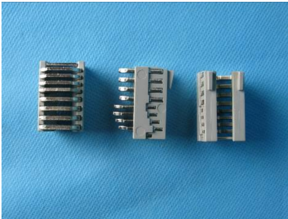
Arc chamber
