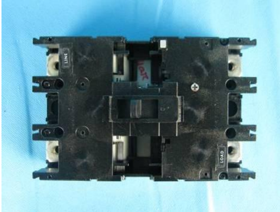
Open view, 2P, MCCB
