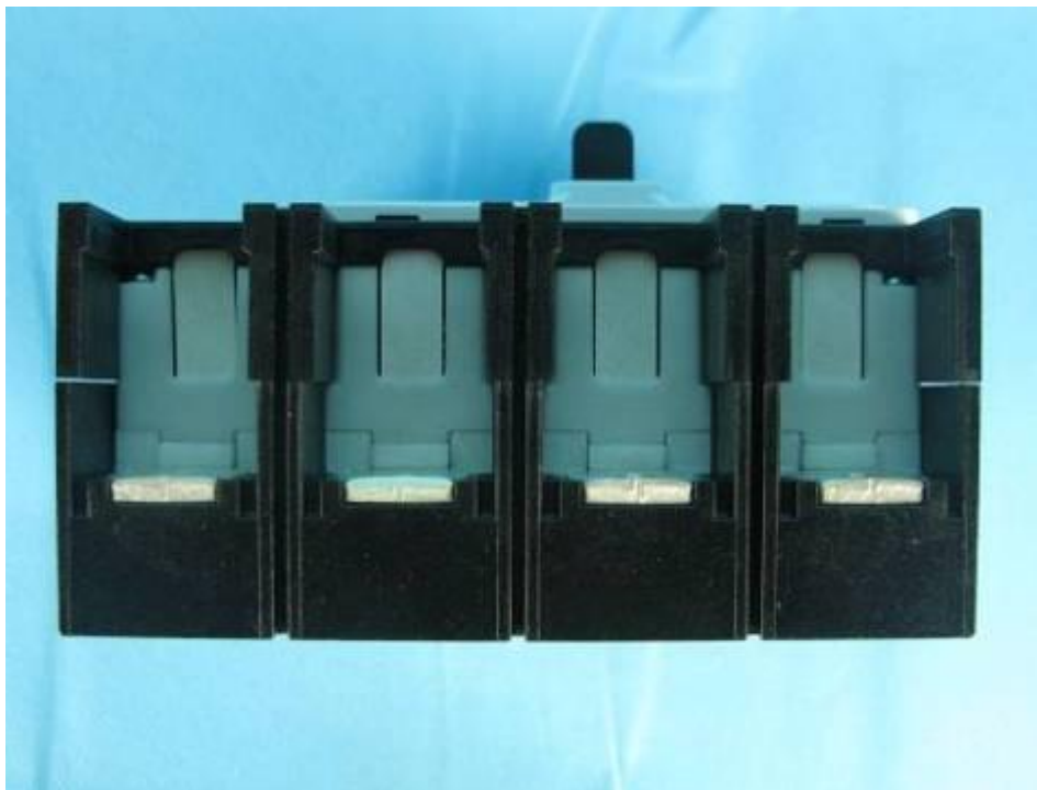
Line terminal view, 3P + N, MCCB
